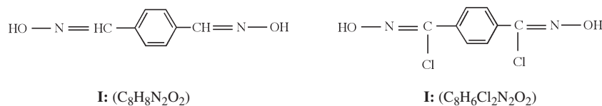
Figure 2. Structures of terephthalaldoxime and terephthalohydroximoyl chloride
